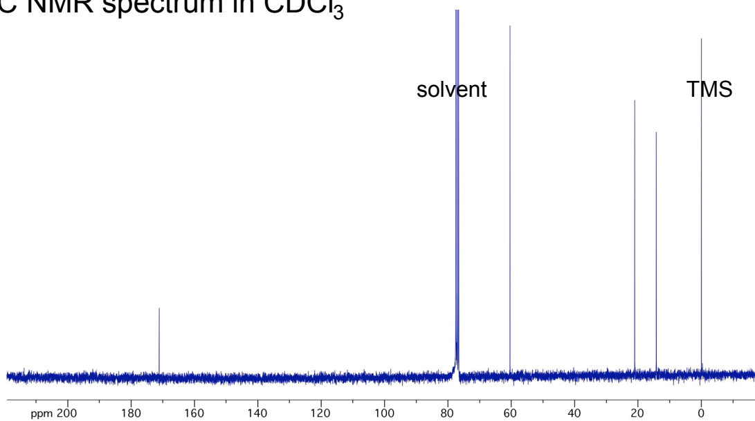
^{13}\text{C} NMR spectrum in \text{CDCl}_3
