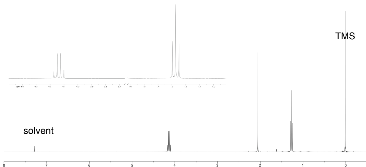
^1\text{H} NMR spectrum in \text{CDCl}_3
